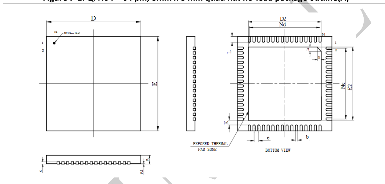
Figure 7-1: QFN64 – 64 pin, 8mm x 8 mm quad flat no-lead package outline(A)
