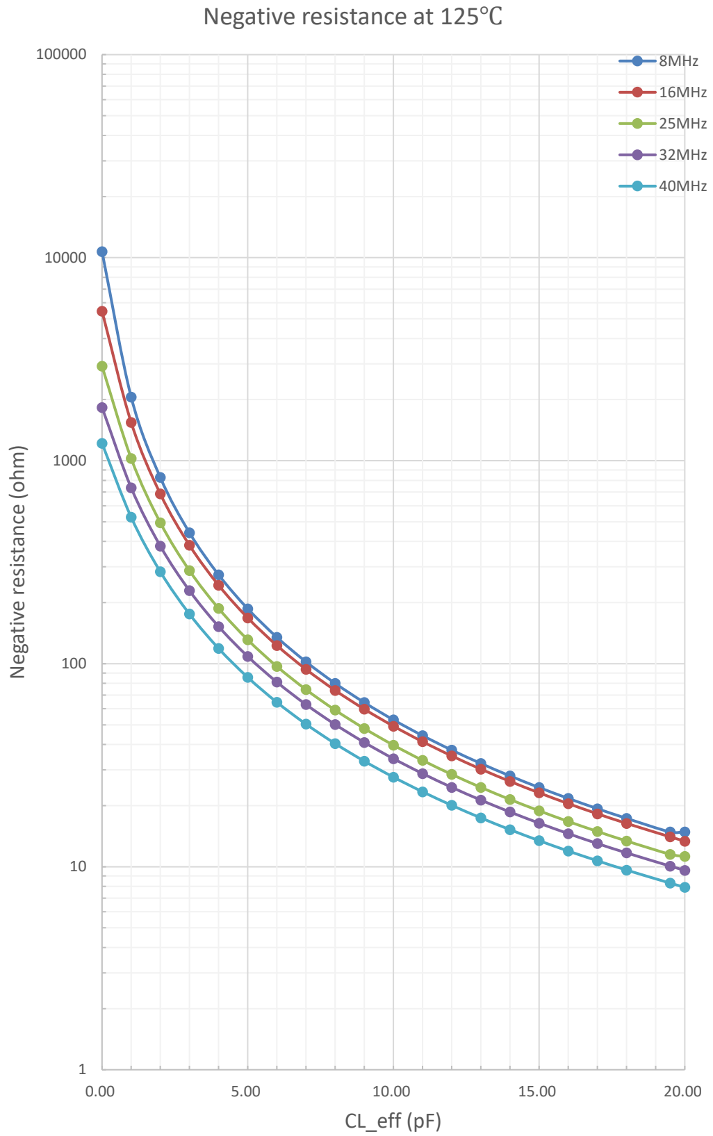
Figure 5-7: The negative resistance of the on-chip crystal oscillator at 125°C
