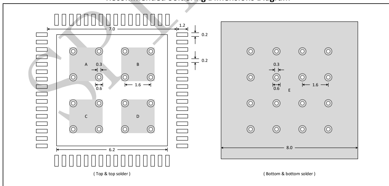
Figure 7-3: QFN64 – 64-pin, 8mm x 8mm Quad Flat No-lead Package Land Pattern and Recommended Soldering Dimensions Diagram
