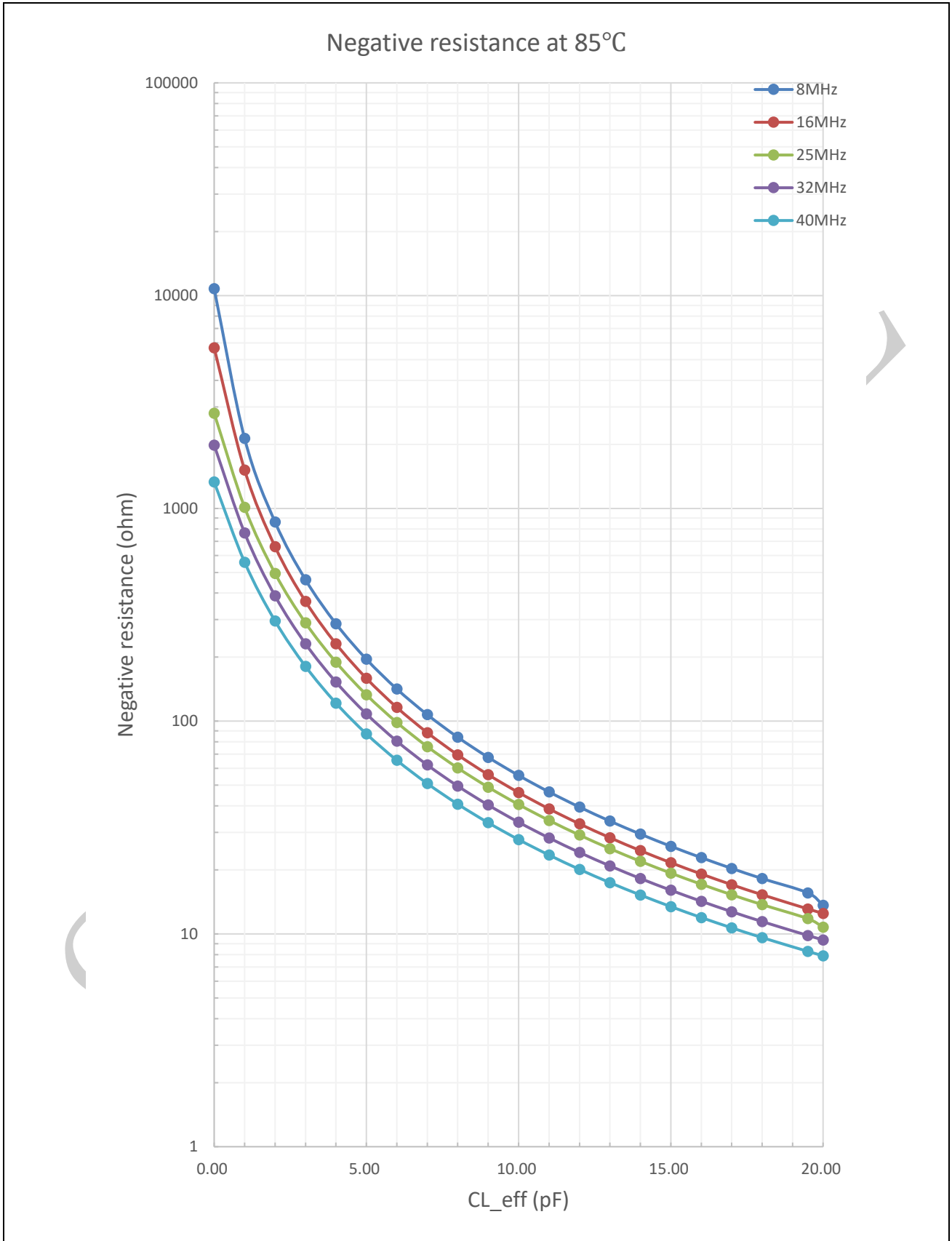
Figure 5-5: The negative resistance of the on-chip crystal oscillator at 85°C
