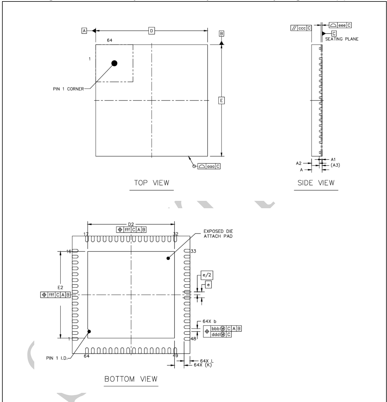
Figure 7-2: QFN64 – 64 pin, 8mm x 8 mm quad flat no-lead package outline(B)
