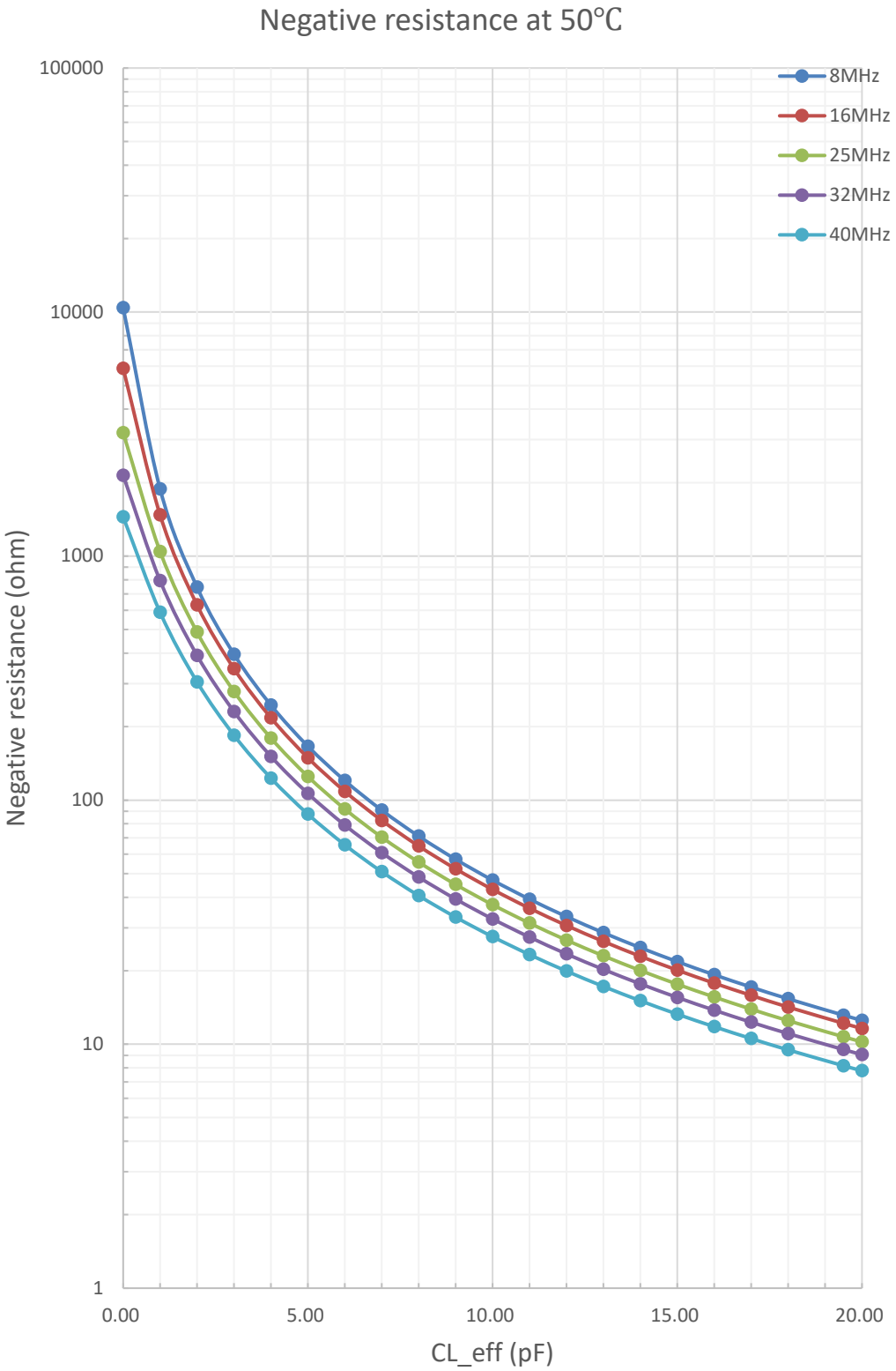
Figure 5-4: The negative resistance of the on-chip crystal oscillator at 50°C
