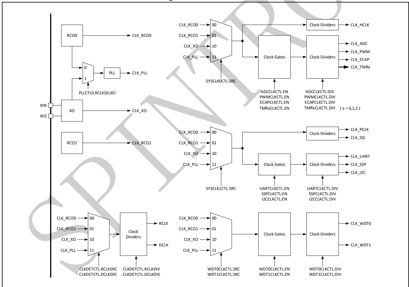
Figure 2-1: Clock tree
