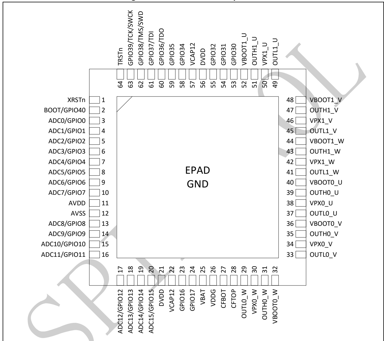
Figure 3-1: SPD1178 QFN64 pin-out
