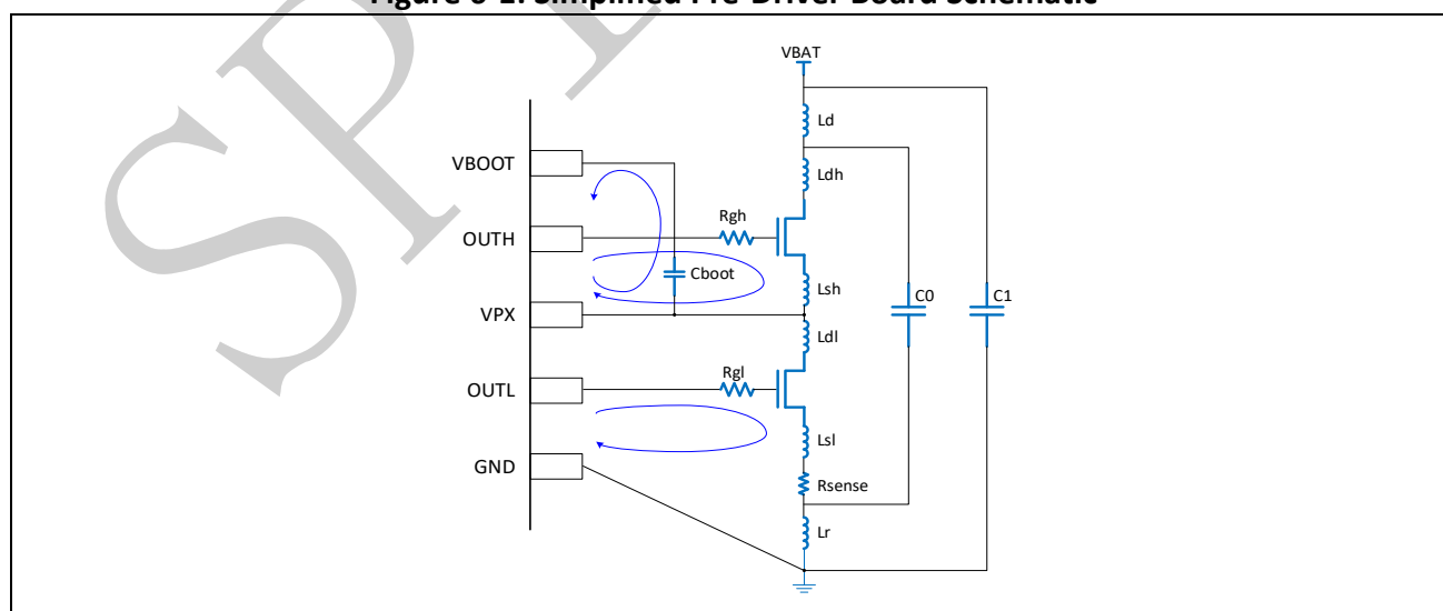
Figure 6-1: Simplified Pre-Driver Board Schematic
